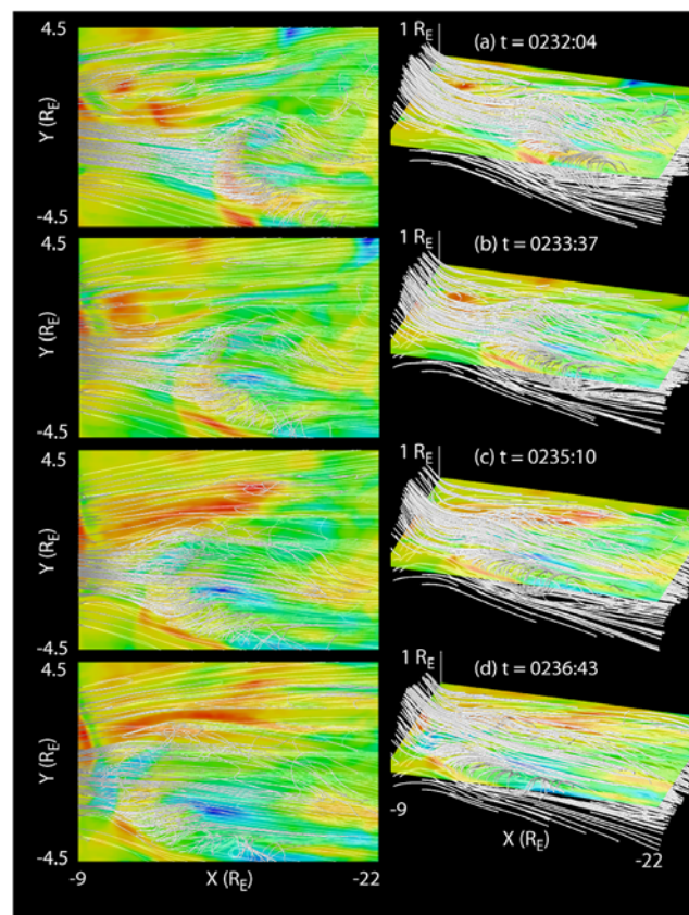
Figure 6. Field line mapping and the equatorial plasma pressure as seen (left) from the top and (right) from the duskside showing the development of a small-scale ( 6 R_E wide and 0.5 R_E in height) earthward moving flux rope that impacts the inner edge of the plasma sheet. This impact leaves the field lines to be directed more vertically, i.e., more dipole-like. The pressure contours have a floating range so that local maxima relative to the position of the flux rope can be seen. These maxima occur with the flux rope but also toward the dawnside.
