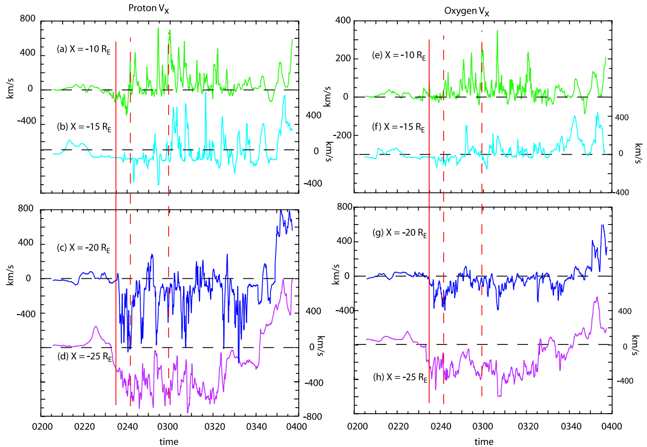
Figure 15. Evolution of (left) the proton and (right) the oxygen x component of the velocity at the four positions downtail used in Figure 5. The time of X line formation is indicated by the solid vertical line, and pseudobreakup and onset are indicated by the dashed vertical lines. The horizontal dashed lines give the zero for each of the graphs. Fast flows are seen down the tail in association with the formation of the X line. These flows develop several minutes before pseudobreakup and a few tens of minutes before onset. The protons have a speed that is on average twice that of the O^+ ions in the Sun-Earth direction.
