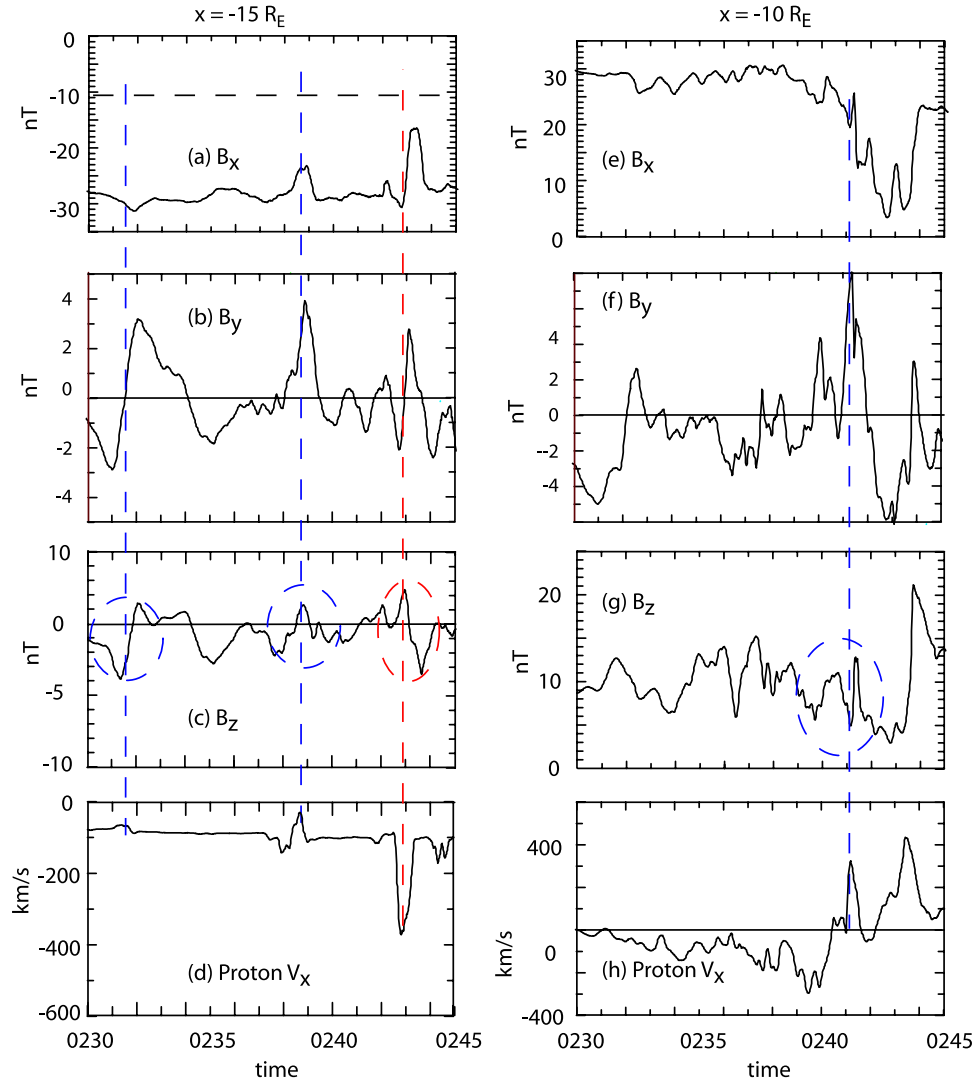
Figure 8. Time histories of B_x , B_y , B_z , and the proton V_x at (left) x = -15 R_E and (right) x = -10 R_E . The earthward moving flux ropes are indicated by the blue dashed circles, and tailward moving flux ropes are indicated by the red dashed circles.
