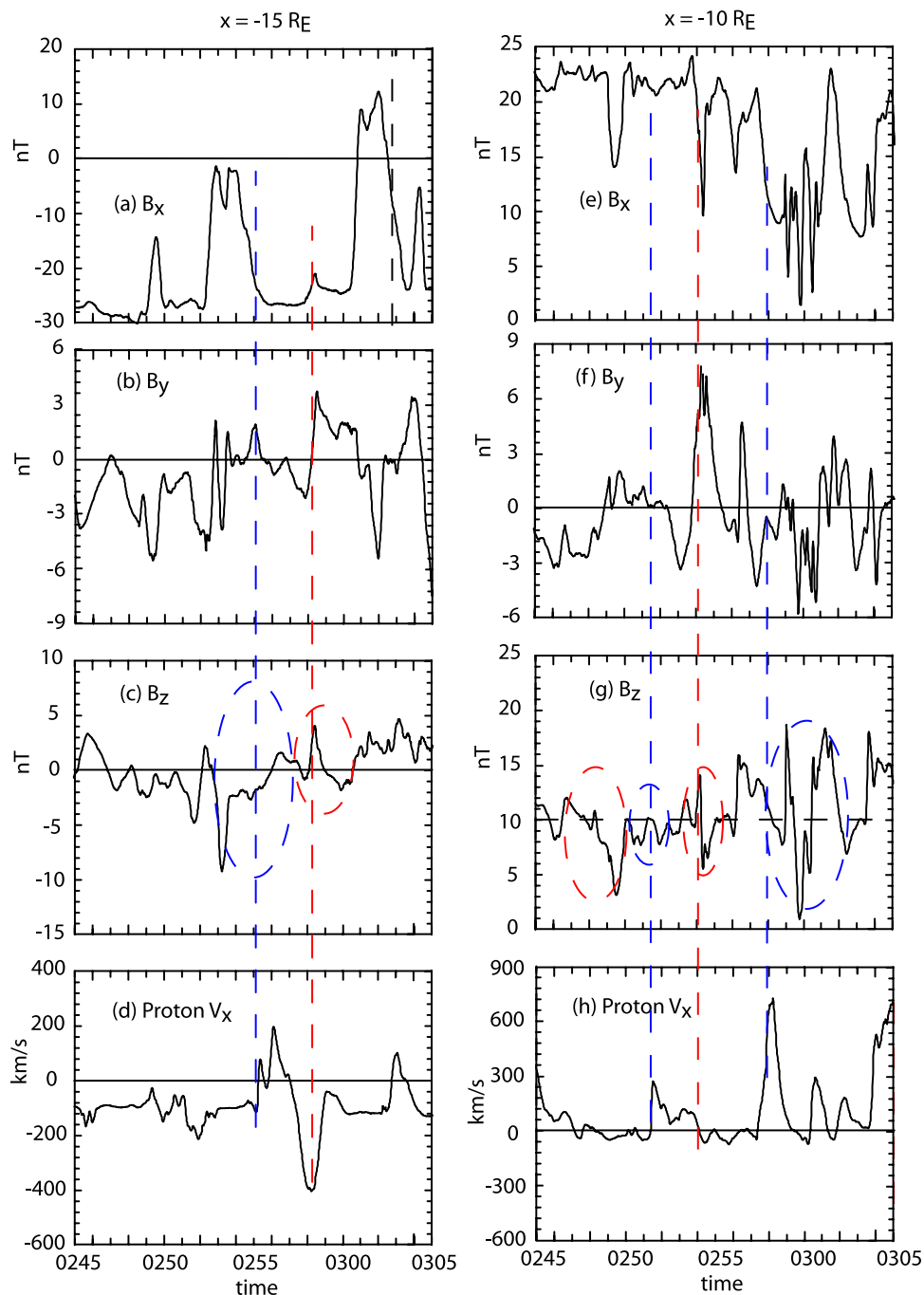
Figure 13. Time histories of B_x , B_y , B_z , and the proton V_x at (left) x = -15 R_E and (right) x = -10 R_E leading up to substorm onset. As in Figure 8 the earthward moving flux ropes are indicated by the blue dashed circles, and tailward moving flux ropes are indicated by the red dashed circles.
