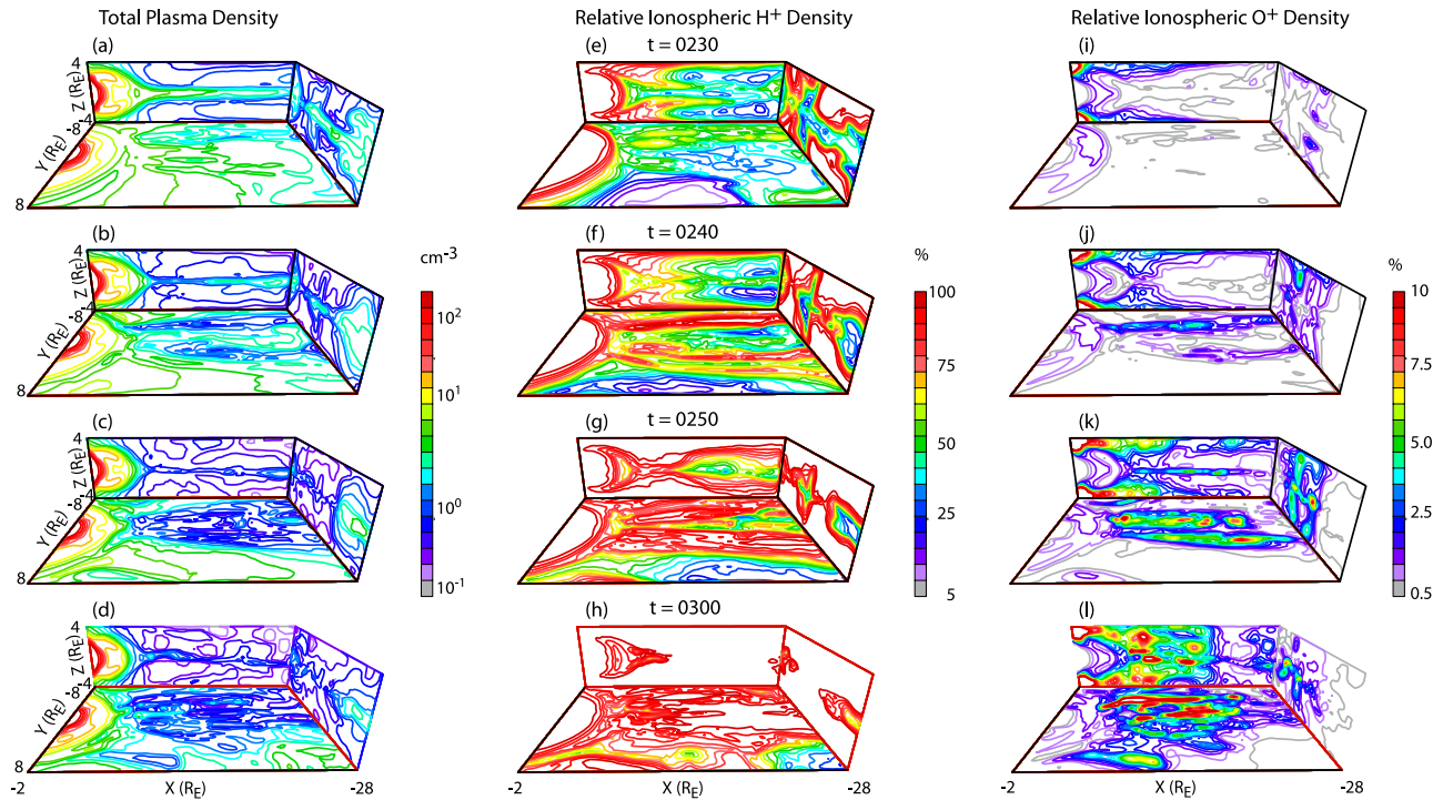
Figure 17. Evolution of the (left) total plasma density, (middle) relative ionospheric H^+ density, and (right) relative O^+ density in the noon-midnight meridian, equatorial plane, and across the tail at x = -20 R_E . The latter is displaced to the right so that the other two views are not obscured. During X line formation, the solar wind plasma dominates the plasma sheet composition. This composition changes to being dominated by ionospheric H^+ around the time of pseudobreakup, with O^+ being a significant factor at substorm onset.
