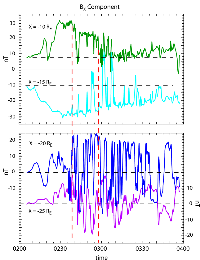
Figure 5. Evolution of B_x at the same four positions in Figure 3. The black horizontal dashed lines show the equilibrium values of B_x prior to the southward turning of the IMF. The red vertical lines indicate the start of a short-lived dipolarization (pseudobreakup) at the spacecraft at 10 R_E . True dipolarization (substorm onset) does not occur until 0258 where B_x returns to its initial value. At larger distances, full dipolarization is not seen. Instead there are multiple and rapid crossings of the plasma sheet which is associated with the kinking of the thin tail current sheet.
