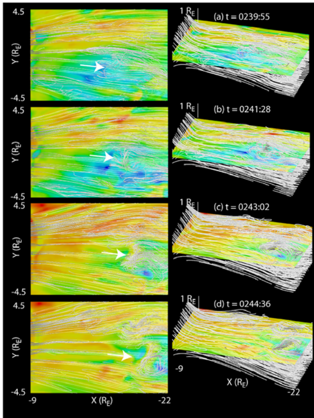
Figure 7. Continuation of Figure 6 showing the development of a tailward moving flux rope, initially forming at x \sim -15 R_E .
