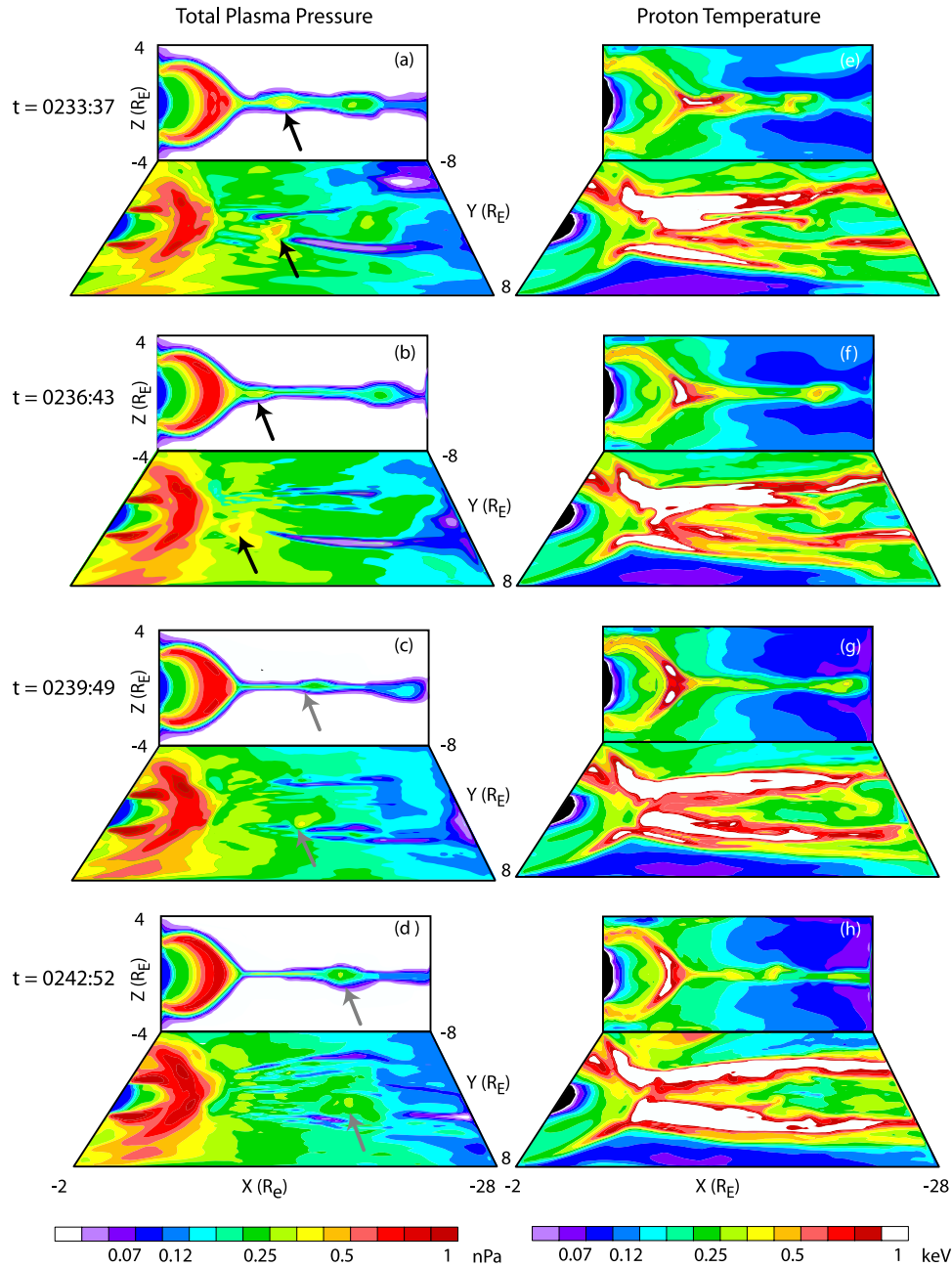
Figure 9. Evolution of (left) the total plasma pressure and (right) the proton temperature in the noon-midnight meridian and equatorial planes. The magnetic field lines out of the auroral zone follow the contours of the plasma pressure in the x - z plane. The earthward moving flux rope is identified by a pressure maximum, as indicated by the black arrows, and is preceded and flanked by hot protons. The impact of the flux rope with the inner edge of the plasma sheet leads to the injection of hot particles up the auroral fields as well as around the dusk and dawn flanks. Reflection of some of the energy leads to the creation of a tailward moving flux rope as indicated by the gray arrows.
