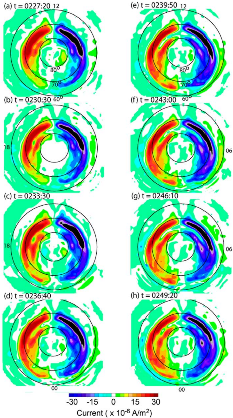
Figure 4. Evolution of the auroral currents. The nightside currents first strengthen along the equatorward edge. At t = 0240 the currents near midnight intensify and expand poleward. This enhanced activity lasts for about 10 min.
