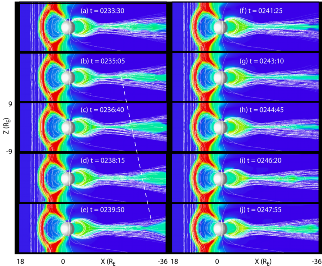
Figure 2. Large-scale view of the evolution of the magnetic field and total plasma pressure through the noon-midnight meridian. An X line forms at t = 0235 in association with the ejection of a plasmoid which is about 10 R_E long. The movement of the rear of the plasmoid is indicated by the dashed white line. In the wake of the plasmoid a Y line forms, where the field lines are essentially parallel to the equator from 10 to 25 R_E and there is transient reconnection that leads to the generation of smaller flux ropes with lengths of 2\text{--}3 R_E .
