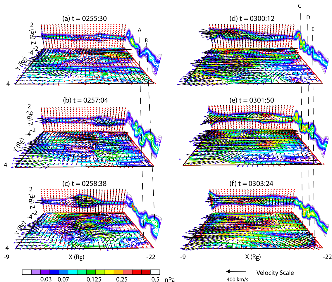
Figure 19. Evolution of the O^+ pressure (contours) and velocity (arrows) during the development of the earthward moving flux rope that produces substorm onset. Red-tipped arrows indicate tailward flow, whereas blue-tipped arrows indicate earthward flow. The passage of the earthward moving flux rope (which is seen as a bulge in the plasma pressure) leads to enhanced O^+ contributions to the overall pressure in the plasma sheet, so that O^+ has a nonnegligible contribution to onset. The black dashed lines show the propagation and evolution of the kinks as they move in the dawn-to-dusk direction.
