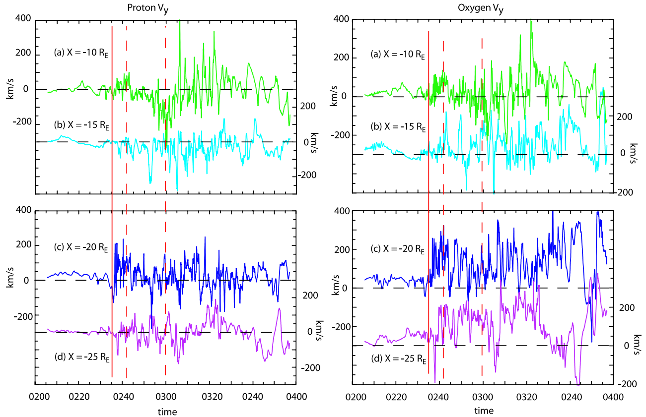
Figure 16. The evolution of V_y for H^+ and O^+ ions in the same format as Figure 15. In this case the O^+ ions have the greatest speed in the dawn/dusk direction, indicating that they are important current carriers.
