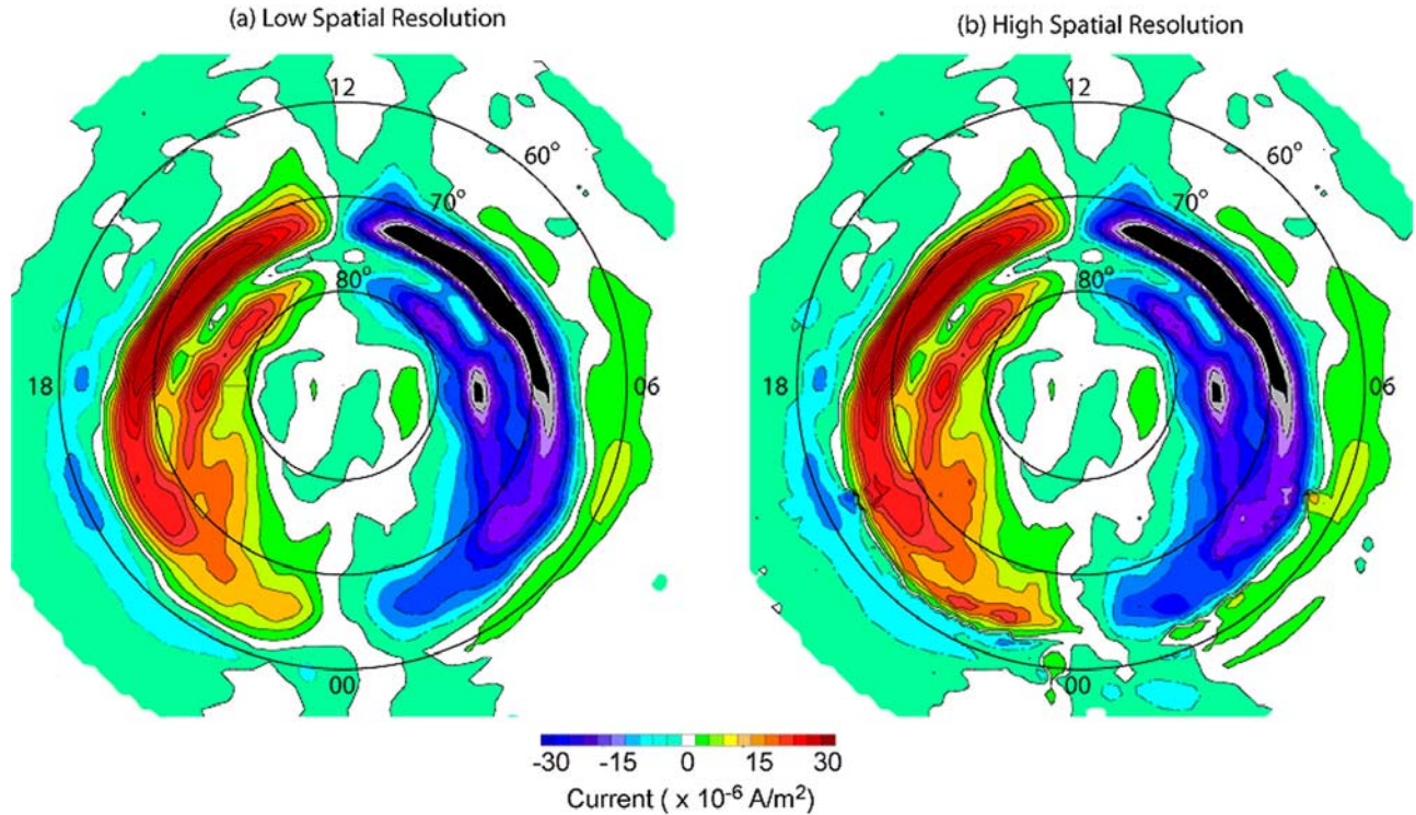
Figure 1. Comparison of the auroral currents using (a) only the base grid system with 1800 km resolution and (b) using the refinement grids with resolution of 450 km at t = 0246 . With the increased spatial resolution more intense auroral currents near midnight are obtained.
