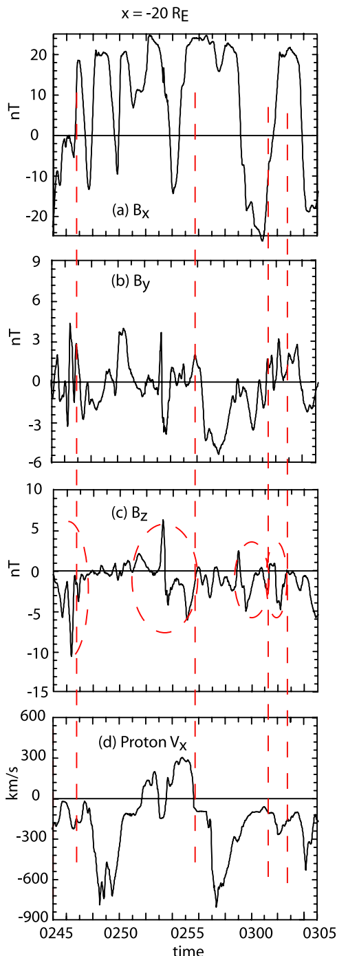
Figure 14. As in Figure 13 but at x = -20 R_E showing the predominance of tailward moving flux ropes and higher-frequency kinking of the tail up to substorm onset.
