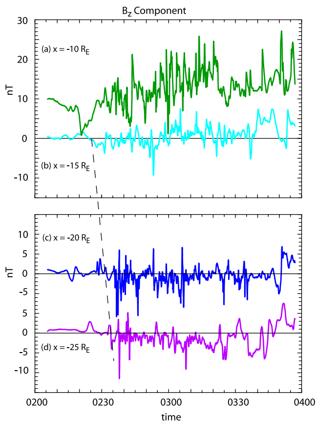
Figure 3. Evolution of B_z at four positions down the tail: (-10, 0., 0.5) R_E (curve a), (-15, 0., -0.5) R_E (curve b), (-20, 0., 0.) R_E (curve c), and (-25, 0., 0.) R_E (curve d). The dashed lines show the propagation of the reconnection down the tail.
