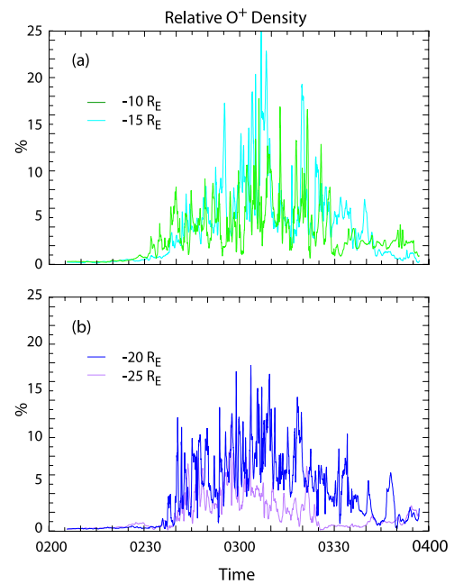
Figure 18. The temporal evolution of the relative O^+ density. Shortly after the formation of the X line, there are enhancements in the O^+ density at x \geq -20 R_E , where the flux ropes develop.
